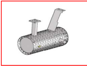
The Catalytic Muffler Part # 37A2-MD seen here is used on a John Deere 2030 Gator
