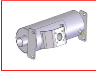
The Catalytic Muffler Part # 3479-MD seen here is used on a Case Skid Steer 410
